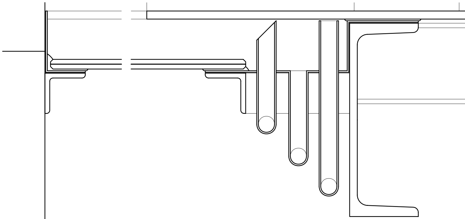
DETAIL OF SECTION
