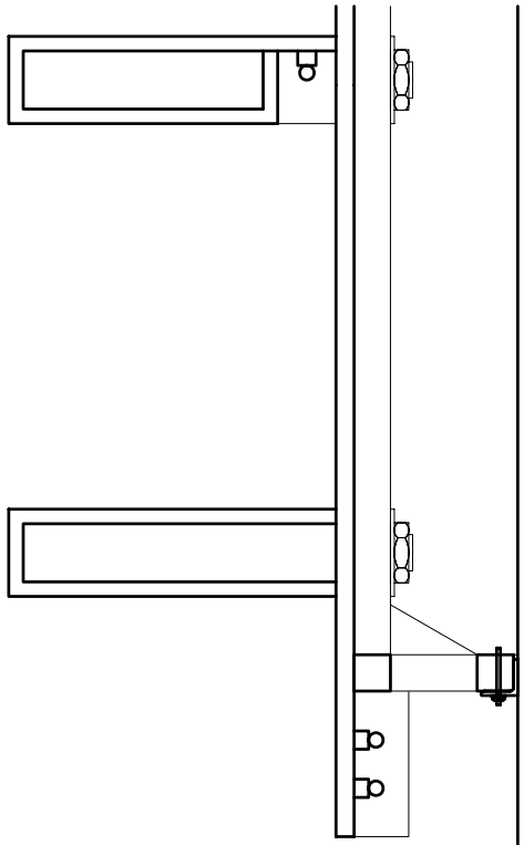
DETAIL OF THE HANGER
