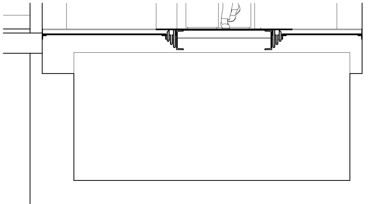
TRANSVERSAL SECTION
